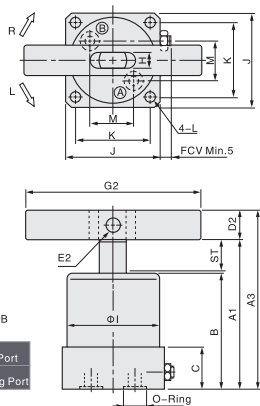
Double side swing clamp
